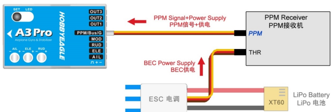
PPM Single-line Connection PPM单线连接
